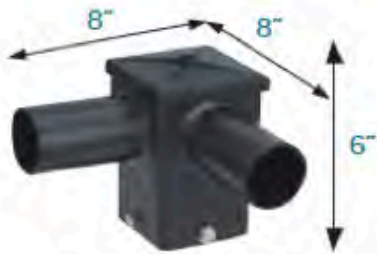
Dual 90° Tenon SKU: TEN-D90
